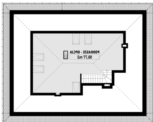
E-112 PODDASZE
